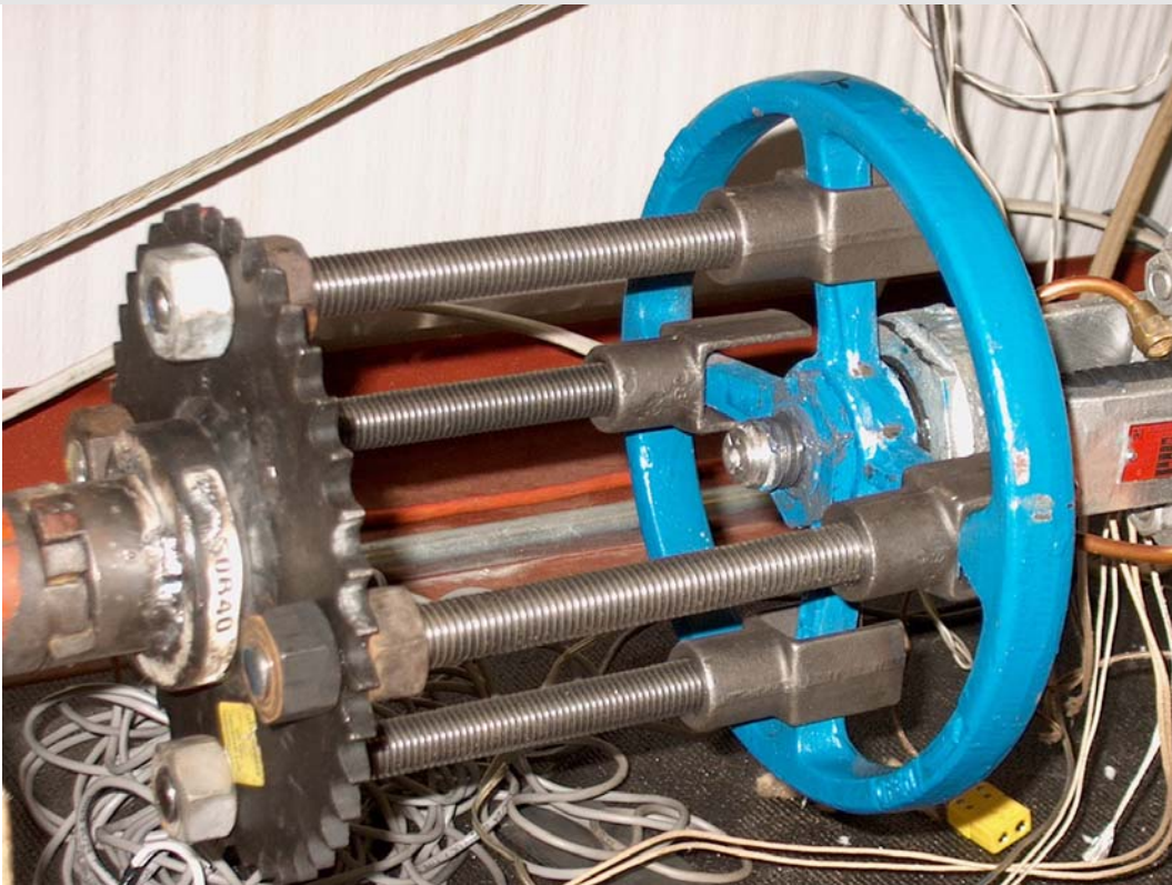
[8] Handwheel Connection
