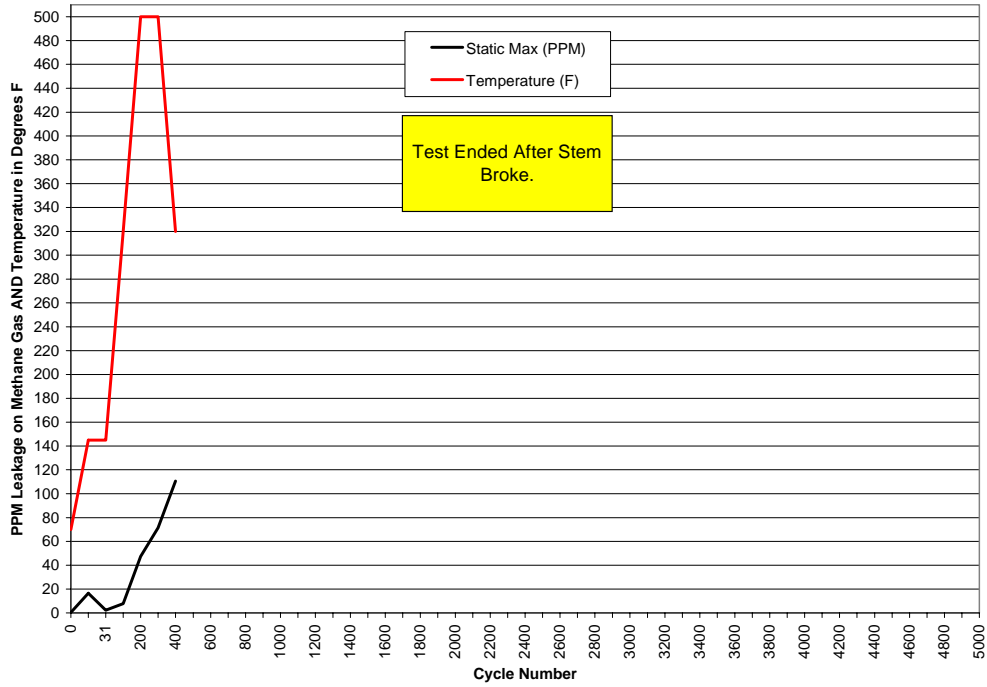
Valve #2, 3/4" Forged Steel Gate Valve
