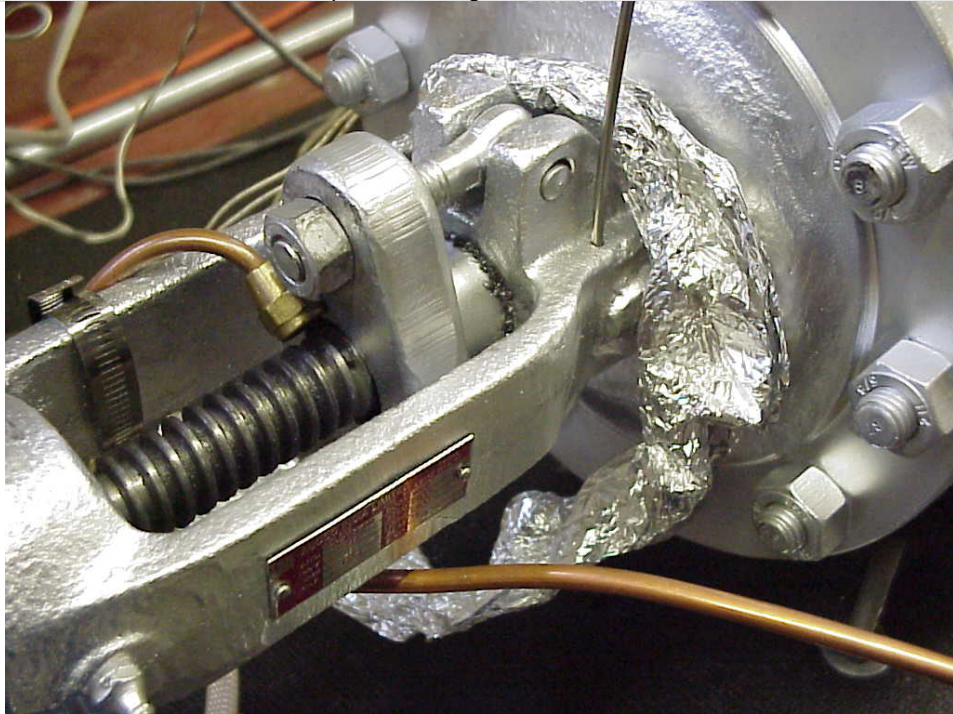
[7] Sample Collection Tube and Thermocouple in Packing Gland
