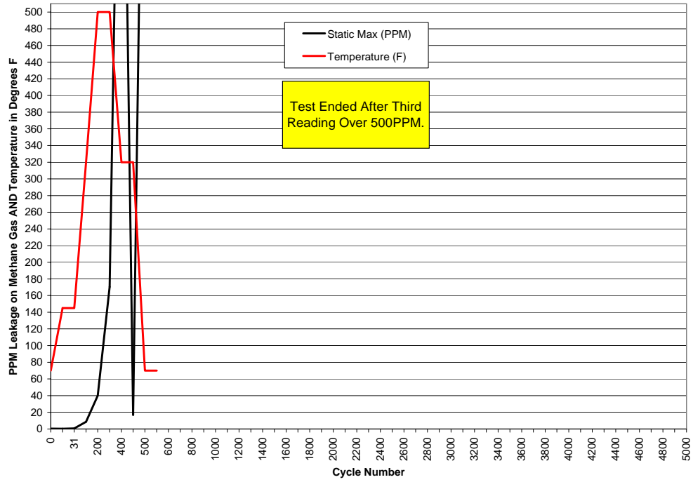
Valve #1, 3/4" Forged Steel Gate Valve
